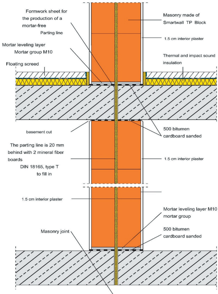
Double-skin house partition
